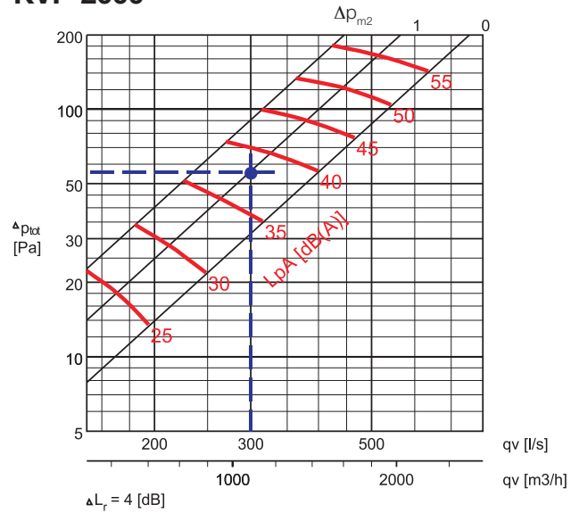
Recommended pressure loss of filter \Delta p_{m1} 35-120 Pa
