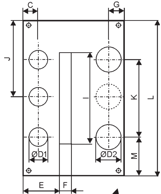
Mounting bracket 150 mm high
